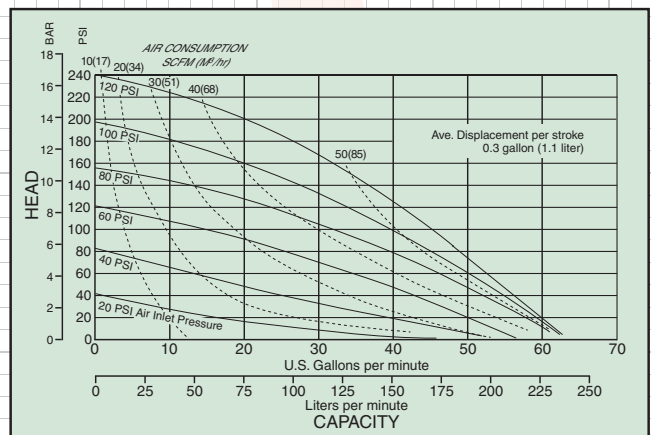
EH2-M & SH2-M Performance Curve
